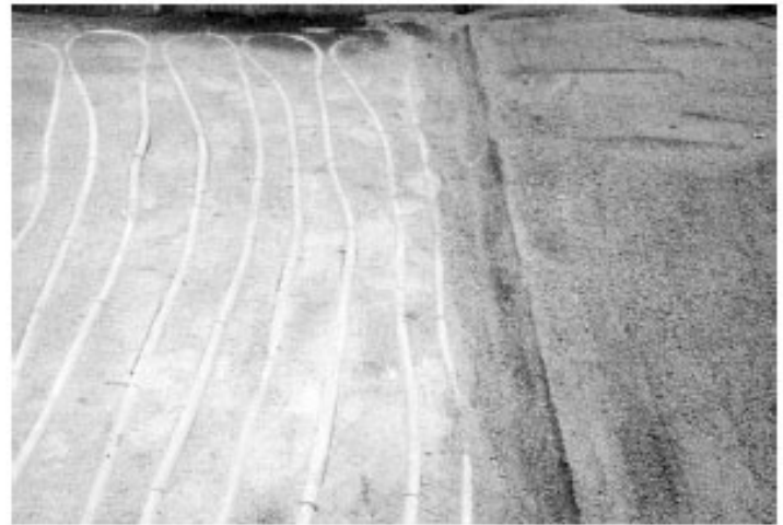
Figure 7. Screeding bedding sand must be done without moving or damaging pipes or wires for melting snow.
