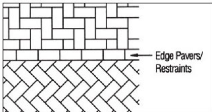
Figure 1. Change in laying pattern direction.
