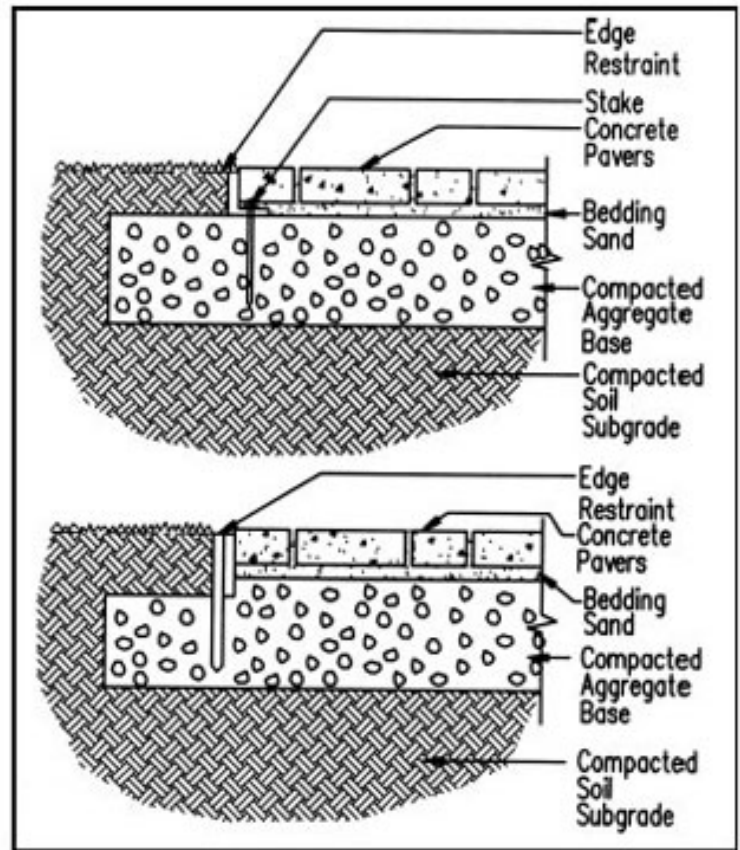
Figure 6. Aluminum and steel edging.
