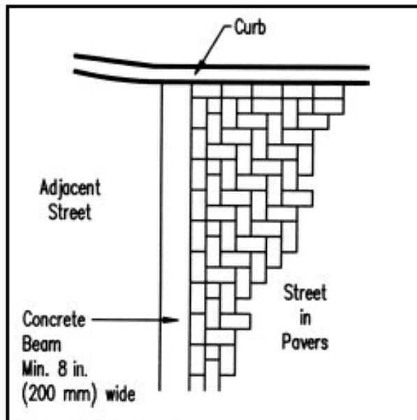
Figure 12. Concrete beam.
