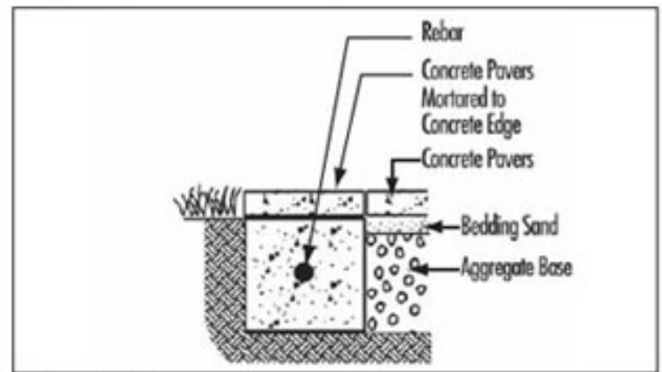
Figure 10. Submerged concrete edge.
