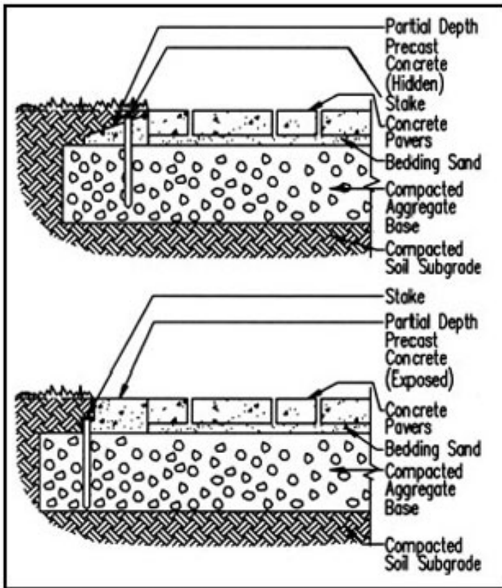
Figure 5. Partial depth precast concrete edge.
