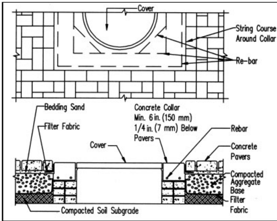
Figure 11. Utility cover.
