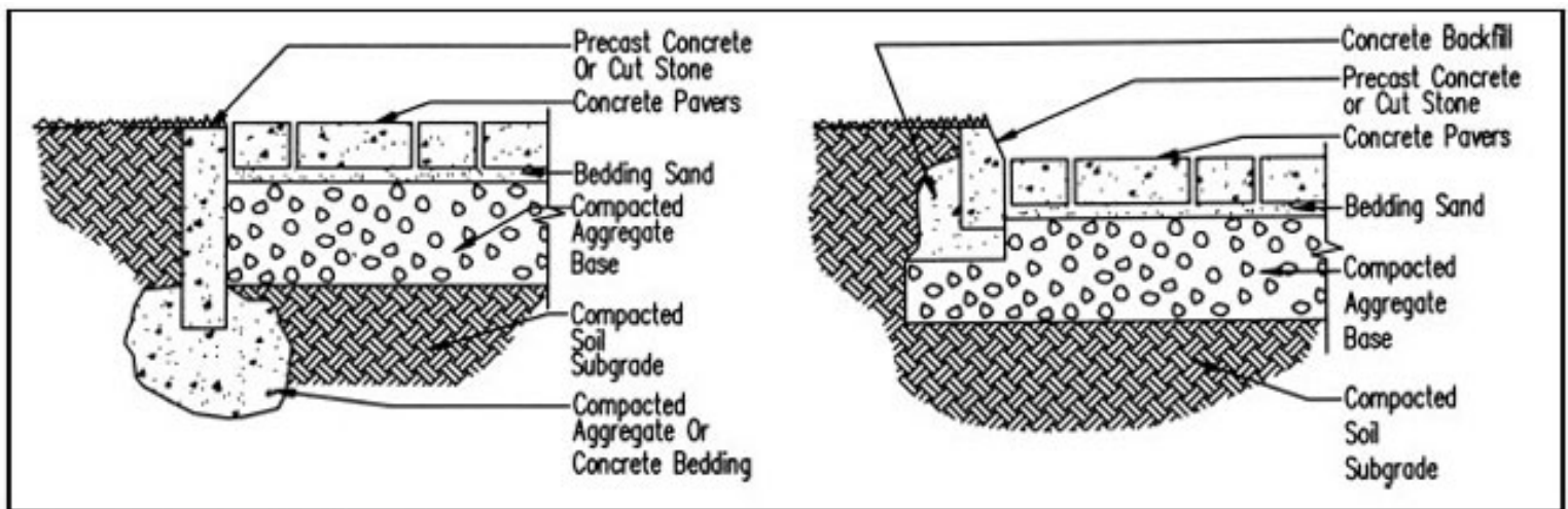
Figure 4. Precast concrete/cut stone.
