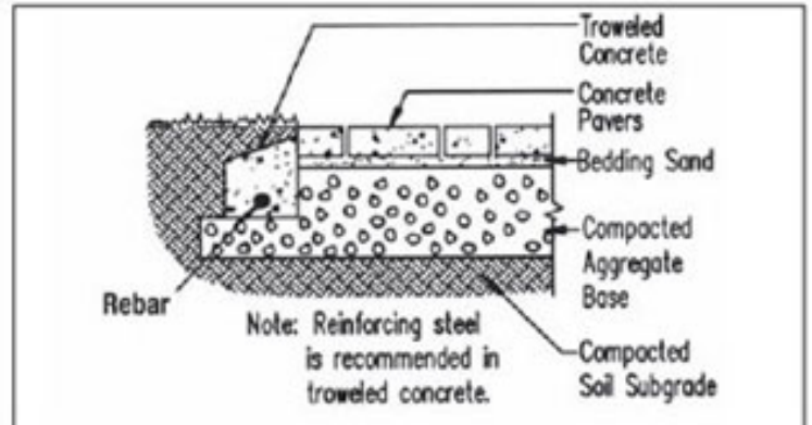
Figure 9. Troweled concrete edges.
