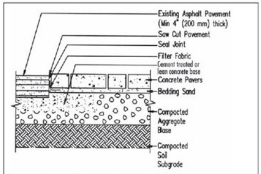
Figure 14. Crosswalk in existing asphalt pavement.
