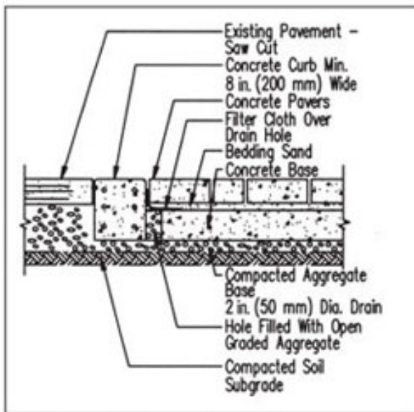
Figure 13. Crosswalk with concrete base.
