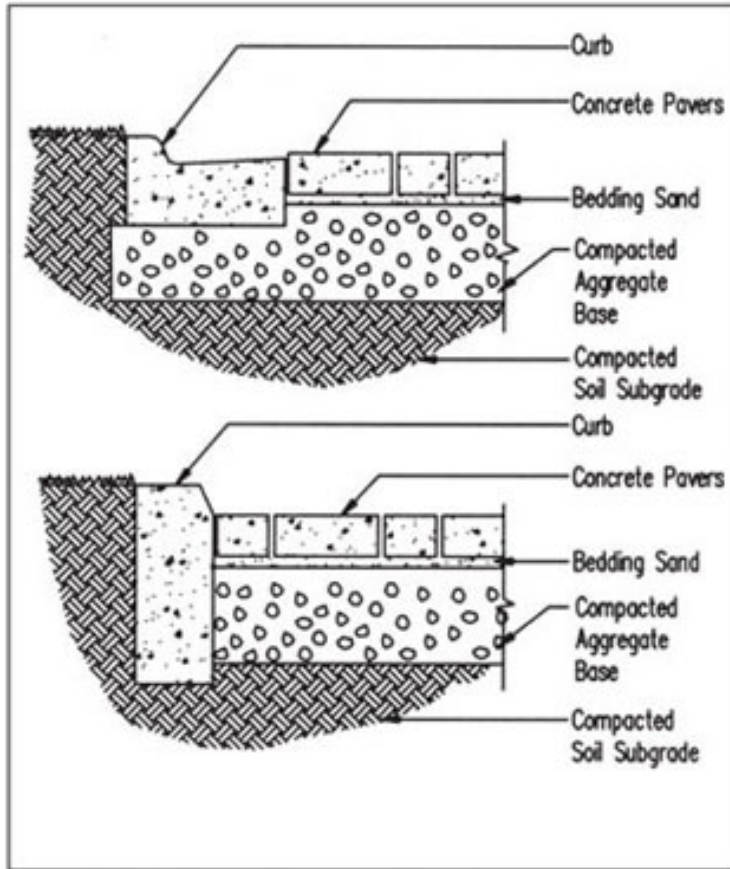
Figure 8. Poured-in-place concrete curbs.
