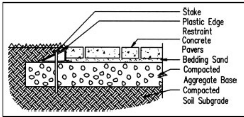
Figure 7. Plastic edge restraint.
